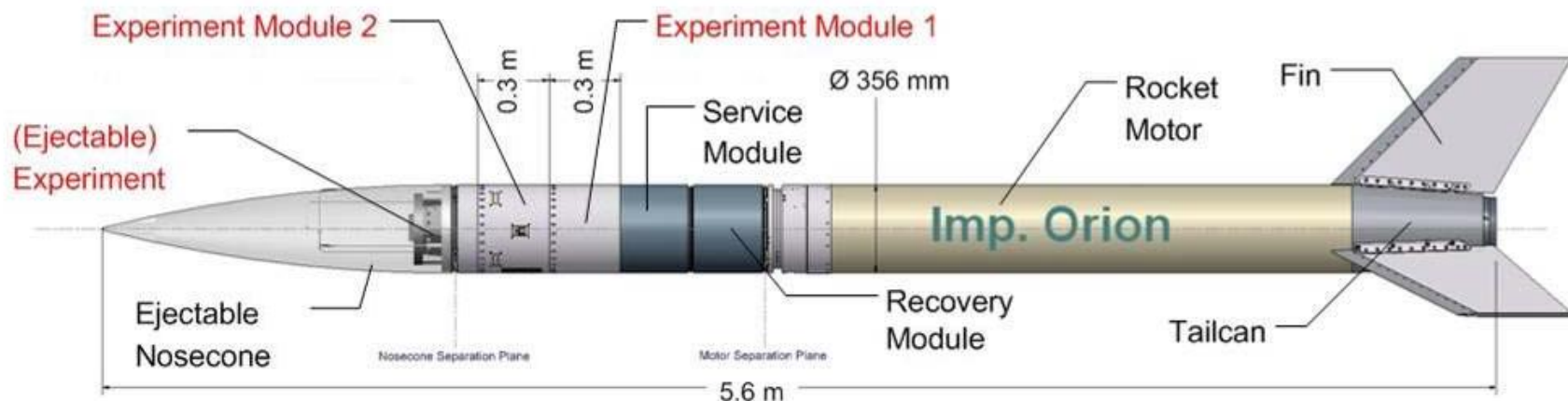
Improved Orion rocket (REXUS system configuration)
