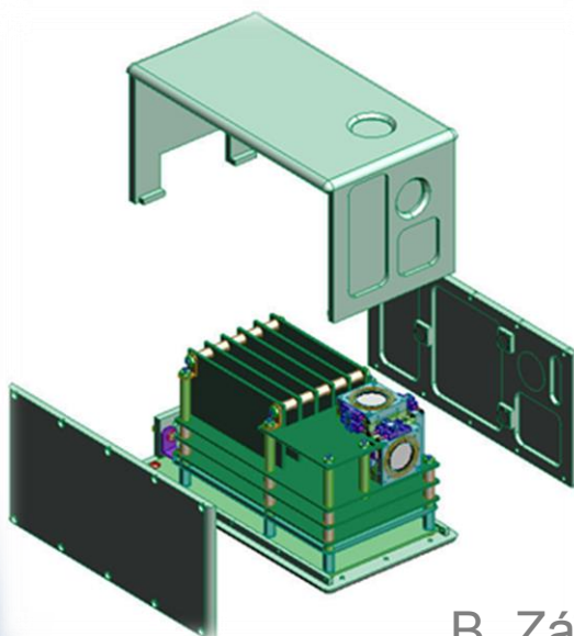
TRITEL 3-dimensional silicon detector telescope system
