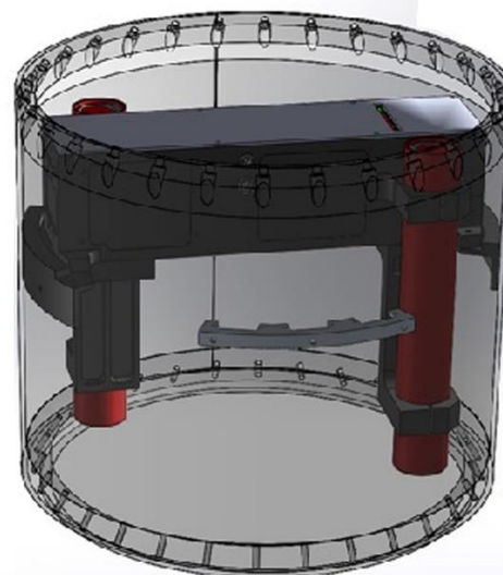
Experiment design and location on-board the rocket
