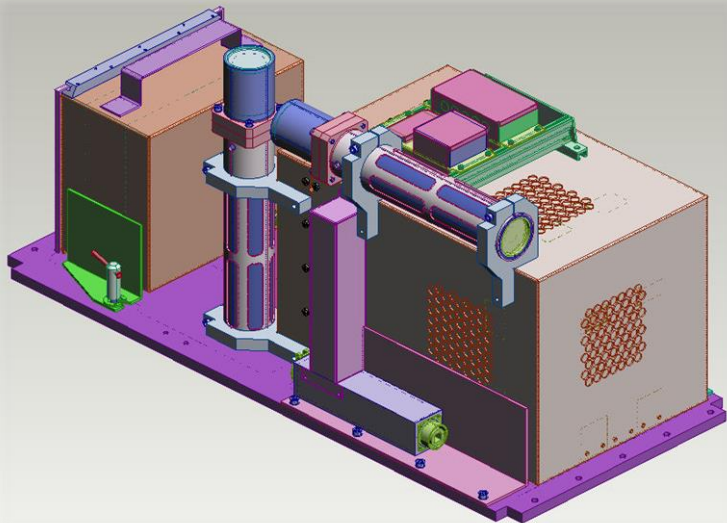
Experiment 3D design model
