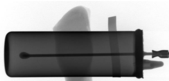
GM tube internal structure in general
