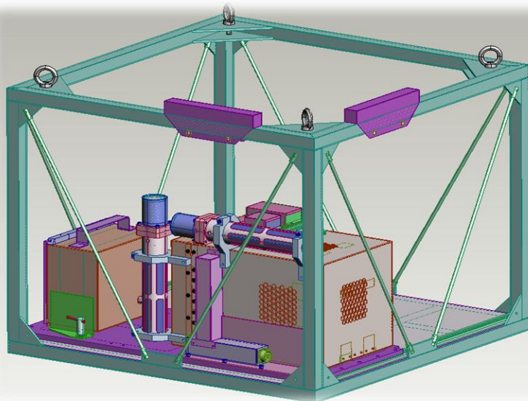
Experiment 3D design model
