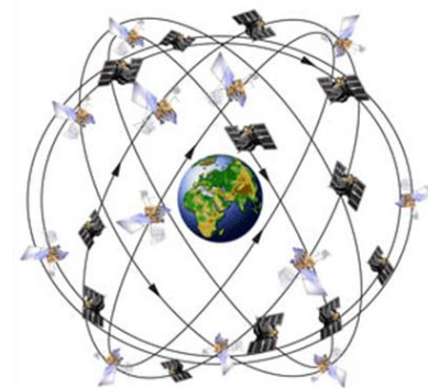
GNSS Constellation
