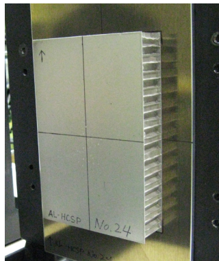
Fig.-5 impact experiment on honeycomb sandwich structure.
