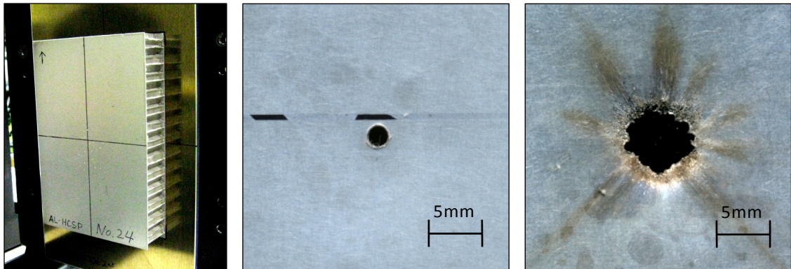
Figure 5 Impact test on a honeycomb sandwich structure: (left) Test setting, (centre) Impacted surface of the honeycomb sandwich panel, (right) Back surface of the honeycomb sandwich panel
