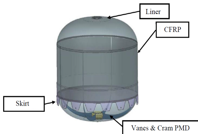
Figure 14 Concept of CFRP propellant tank
