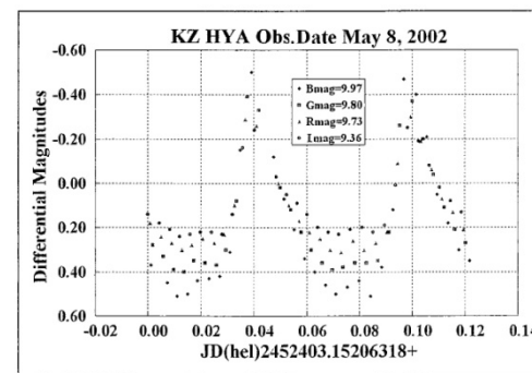
Figure 3. The observation of CCD photometry of the KZ Hya with BGR I colors which were made during the night of May 8, 2002
