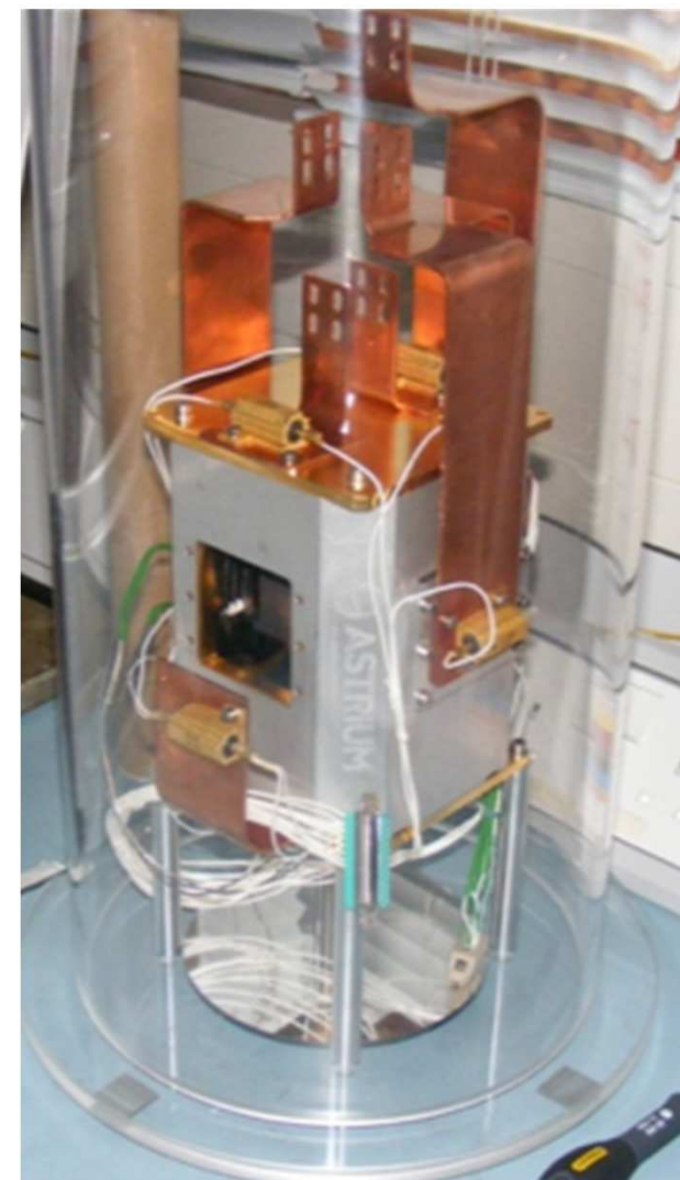
Electrically Heated 5 W RTG Laboratory Prototype (University of Leicester)
